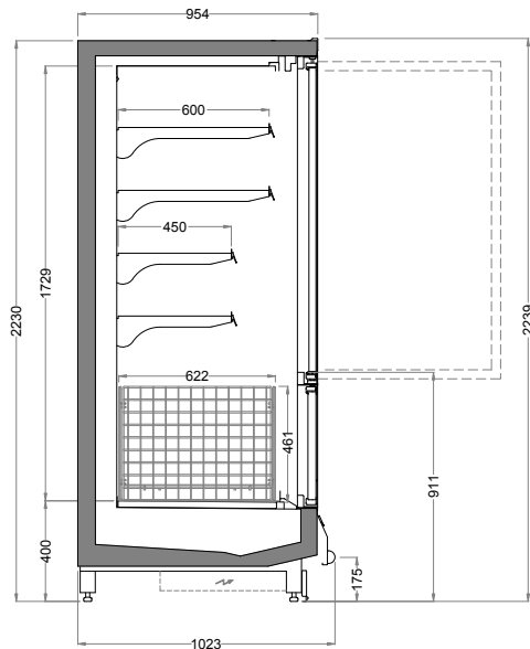
SVEA COMBI 2230
