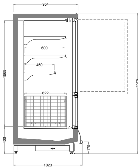
SVEA COMBI 2070
