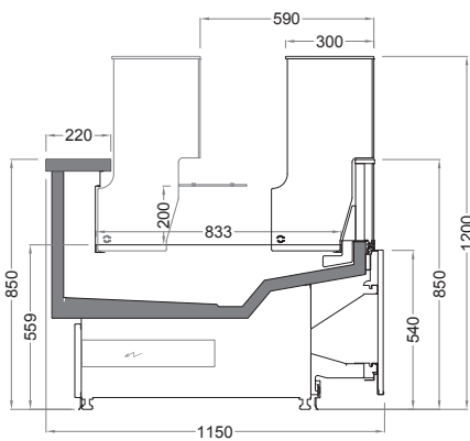
CITRINE CONVERTIBLE 830 / 1200 / 1150 / 540-SQ-AA
