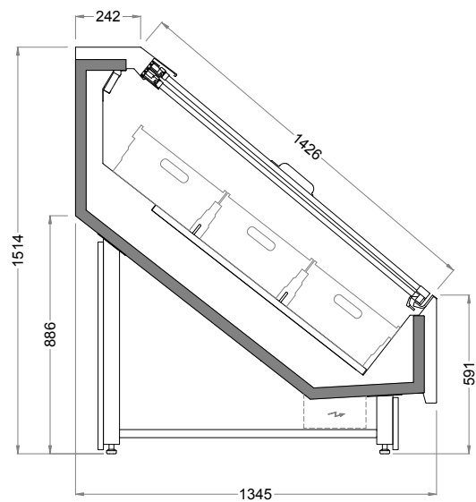
FLORIT with Lids
